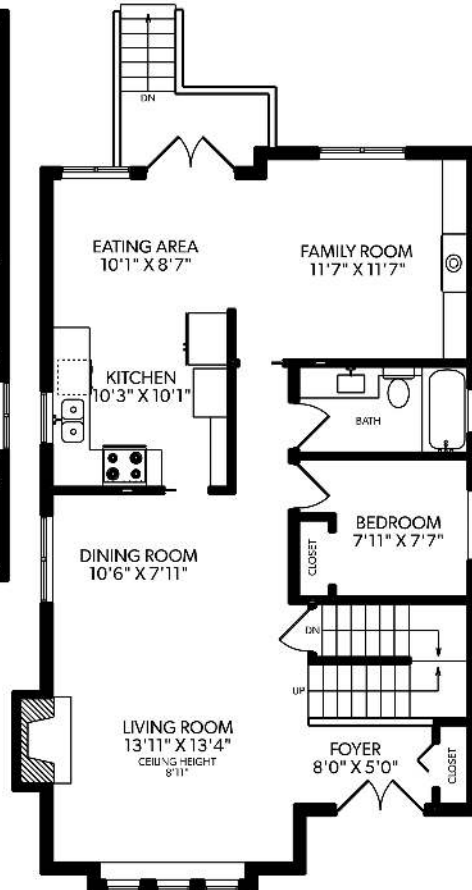
MAIN FLOOR
