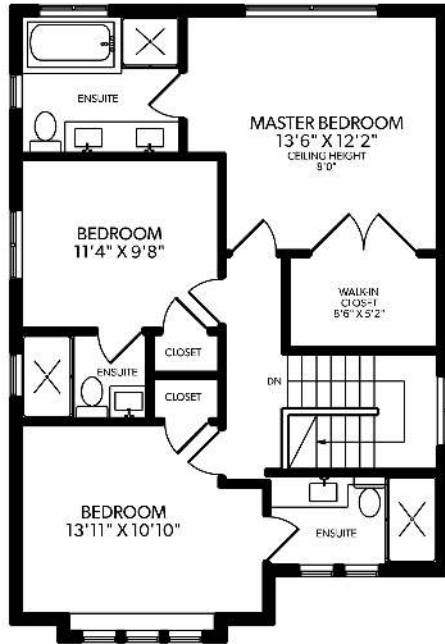
UPPER FLOOR
