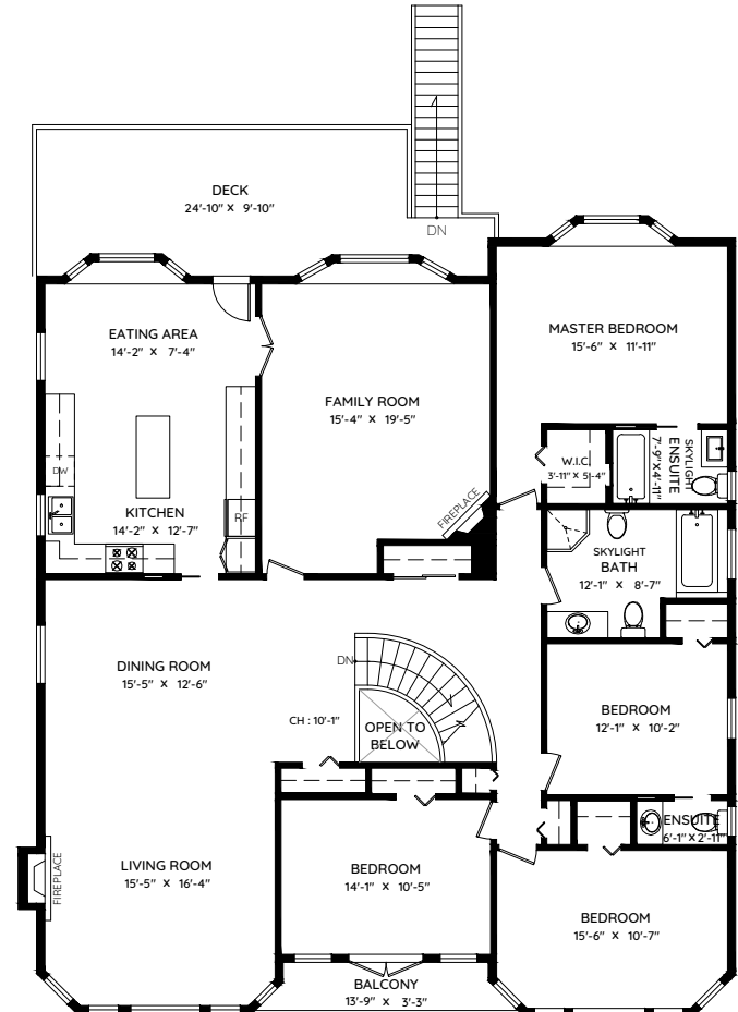
MAIN FLOOR 2,285 SQ.FT. CH: 8'-0"
