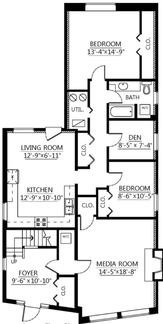
Lower Floor Plan Floor Area: 1,428 sq.ft.
