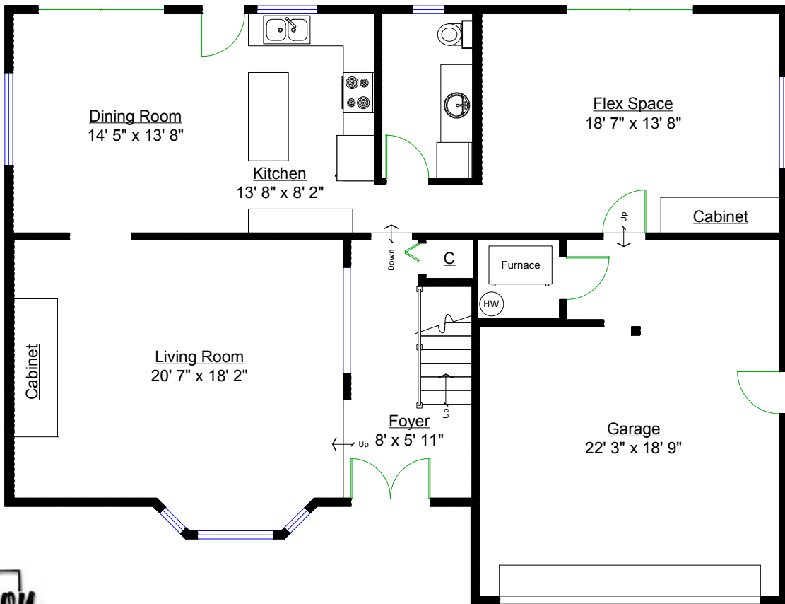
MAIN LEVEL
