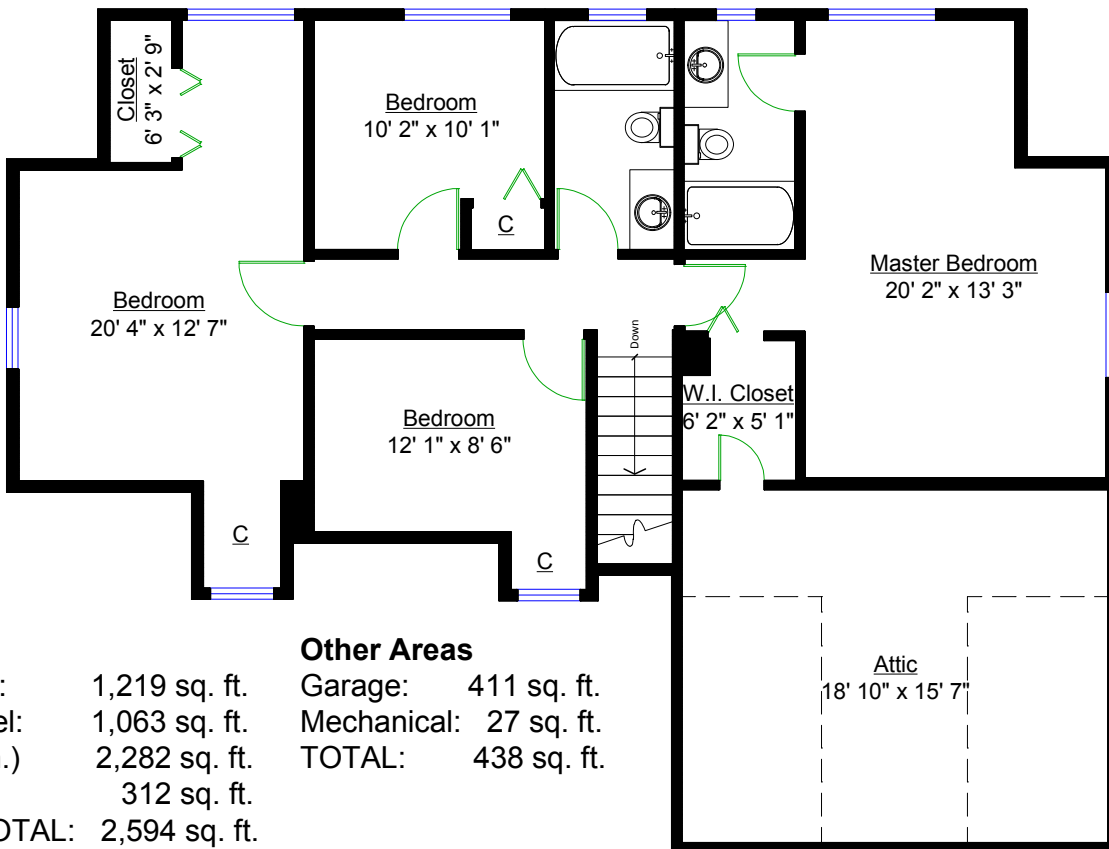
UPPER LEVEL
